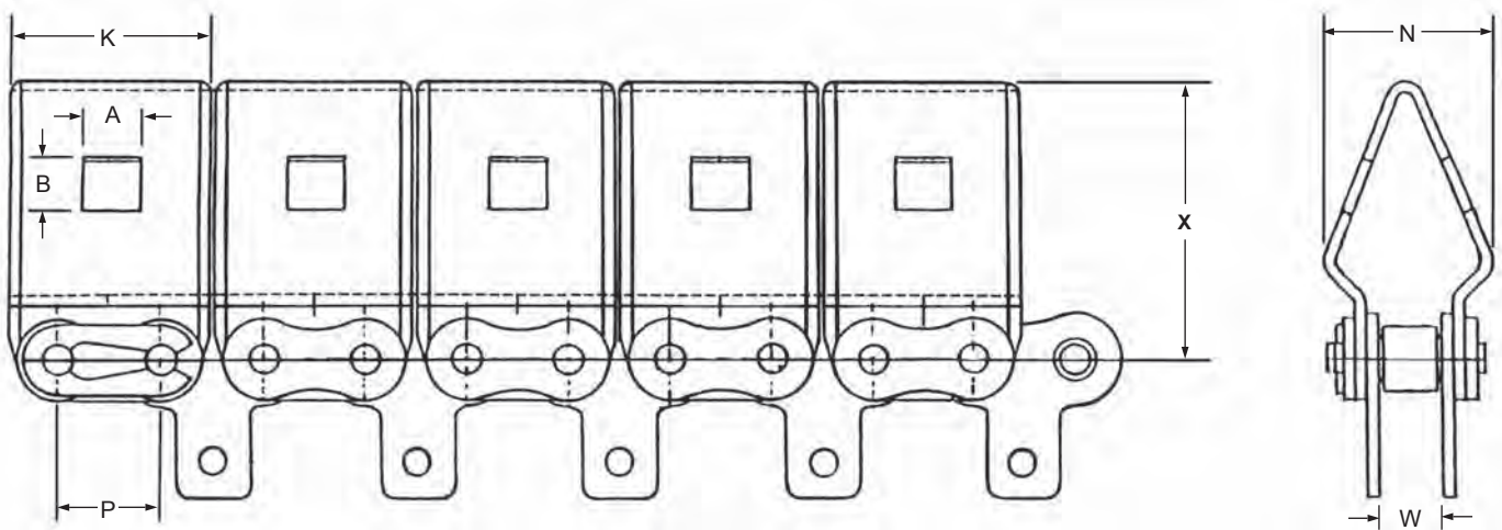
40 BOOK BINDING CHAIN / RIVETED TYPE / SPRING CLIP TYPE
