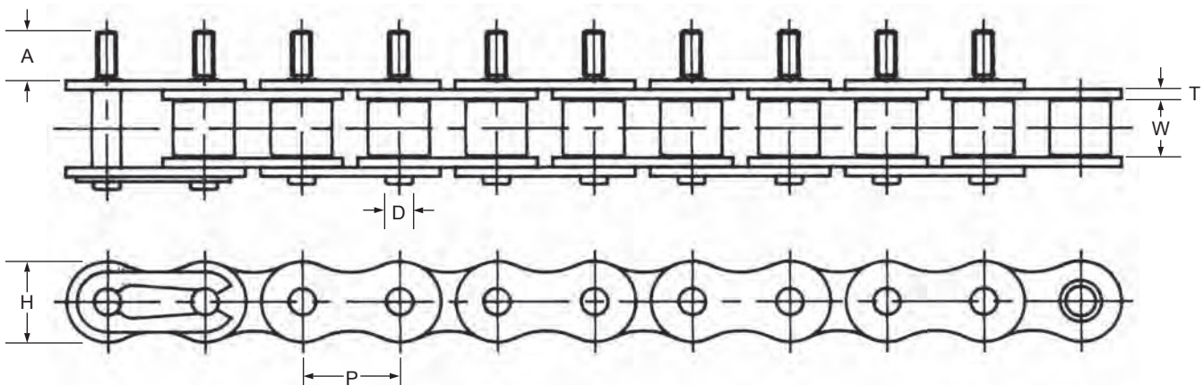
12B BOOK BINDING CHAIN / RIVETED TYPE
