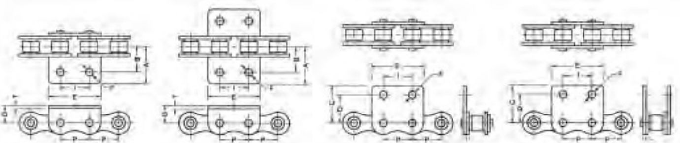
WA-2 / WK-2 / WSA-2 / WSK-2 Attachments
